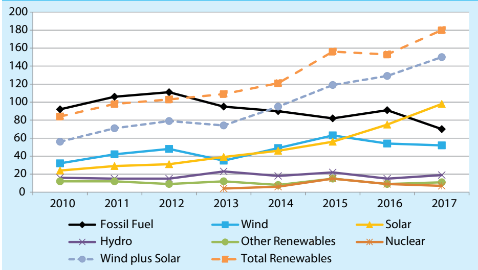
Figure 3: Global Net Capacity Growth in Giga Watt (GW) by Sources, 2010-2017 2
