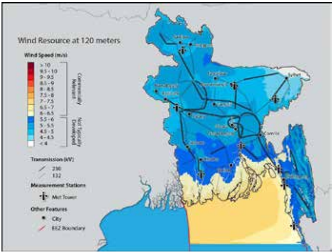
Figure 1: Wind Resource Map of Bangladesh and Measurement Locations 9
