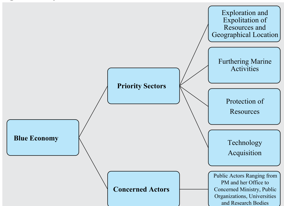
Figure 1: Analytical Framework
